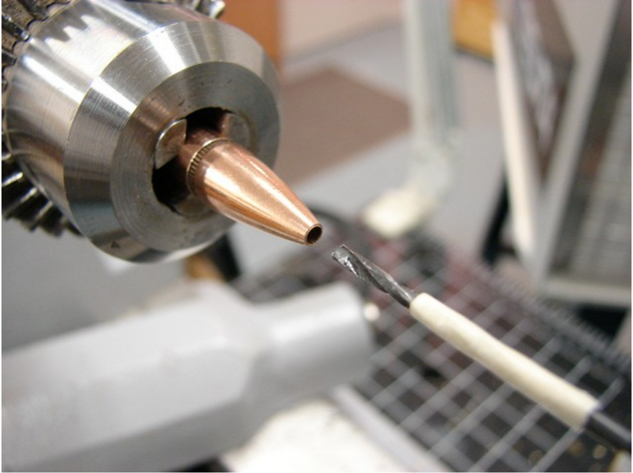
Drilling refill tip hole with #46 bit.
