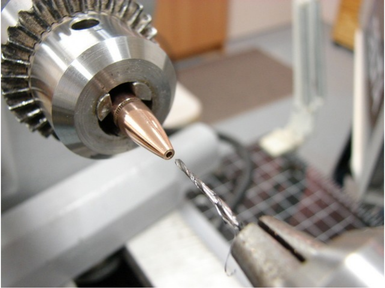
Drilling pilot hole with #55 bit.
