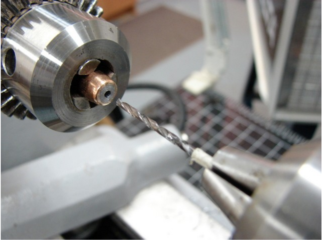
Drilling 5/64th pilot hole.
