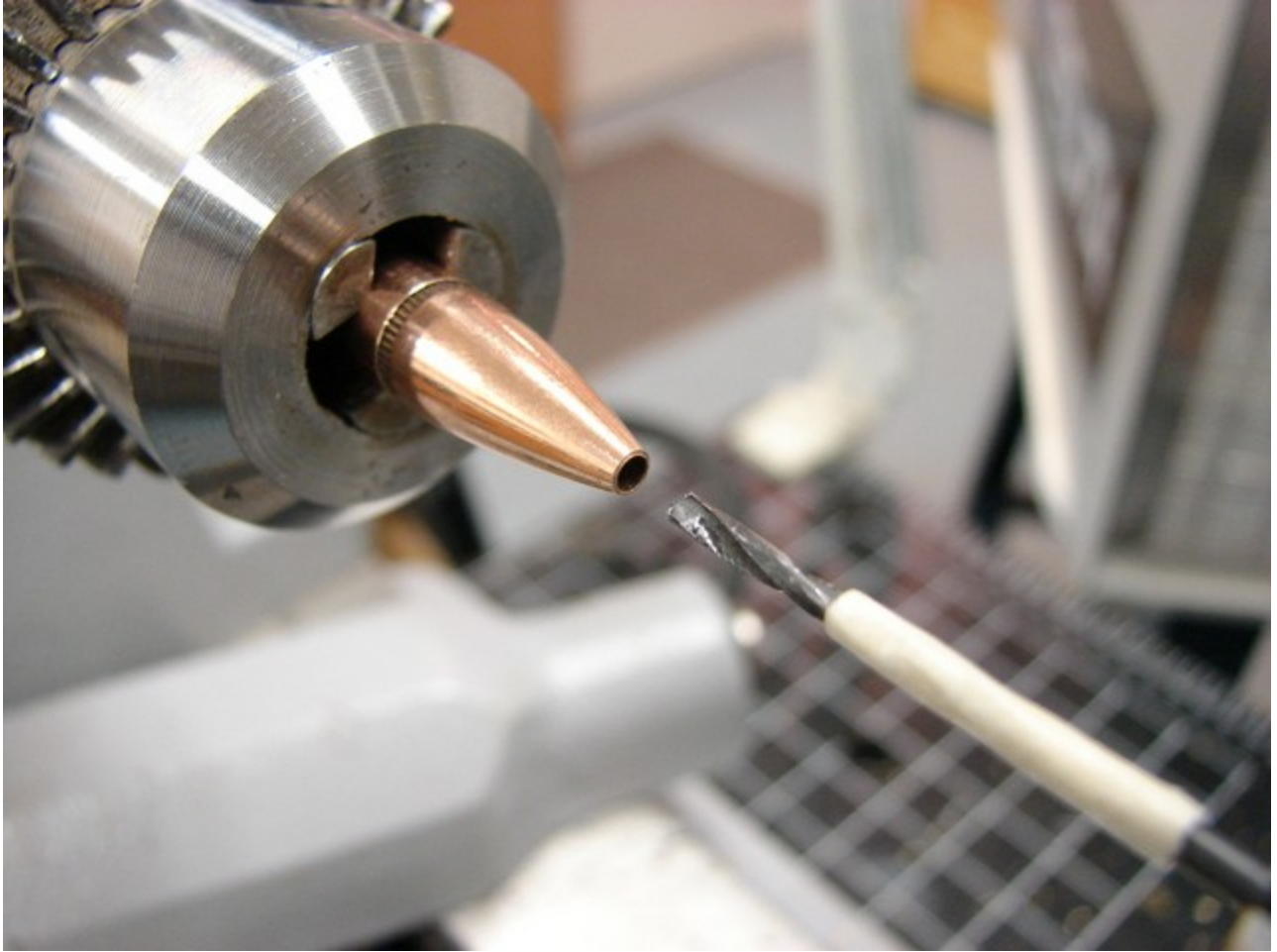
Drilling refill tip hole with #46 bit.
